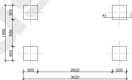
Fundamentplan
